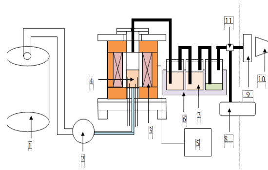
Gambar 1 Instalasi Penelitian
