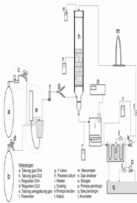
Gambar 1. Instalasi Penelitian
